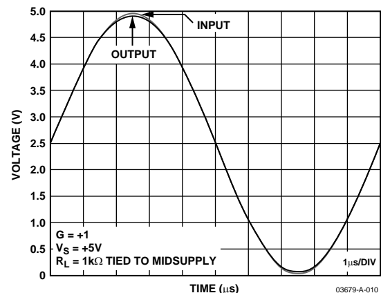
Figure 5. Rail-to-Rail Response
