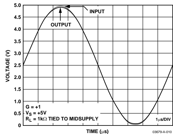
Figure 5. Rail-to-Rail Response
