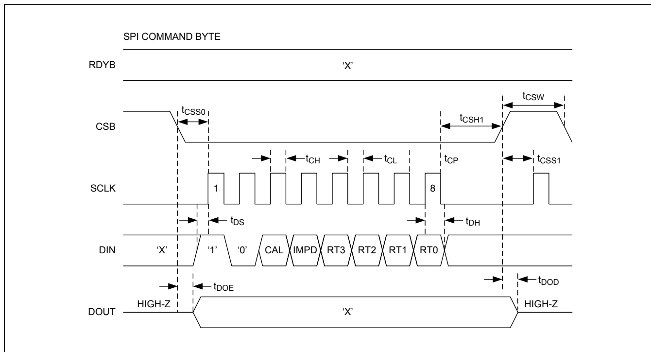
Figure 17. SPI Command Byte Timing Diagram
