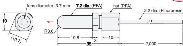
E32-T11F (R4) Free-cut
