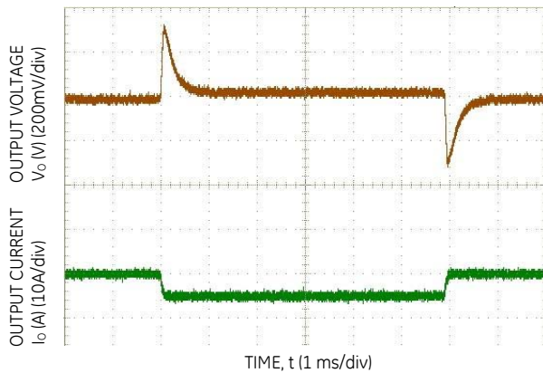
Figure 11. Typical Transient Response to Step Change in Load from 25% to 50% to 25% of Full Load at 48Vdc Input and C_o = 220\mu F Polymer, with -02 option.
