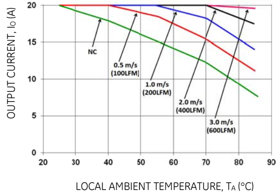
Figure 23. Output Current Derating for the Base Plate EBDW020A0Bxx-H and 0.25" heat sink in the Transverse Orientation; Airflow Direction from Vin(-) to Vin(+); Vin = 48V. Layout Considerations
