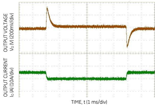
Figure 12. Typical Transient Response to Step Change in Load from 50% to 75% to 50% of Full Load at 48Vdc Input and C_o = 220\mu F Polymer, with -02 option.
