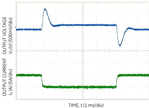
Figure 5. Typical Transient Response to Step Change in Load from 25% to 50% to 25% of Full Load at 48Vdc Input and C_o= 470\mu F Polymer, without -02 option.
