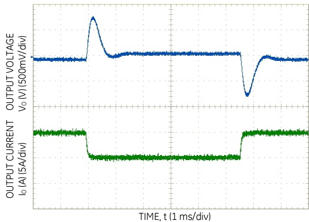
Figure 6. Typical Transient Response to Step Change in Load from 50% to 75% to 50% of Full Load at 48Vdc Input and C_o= 470\mu F Polymer, without -02 option.
