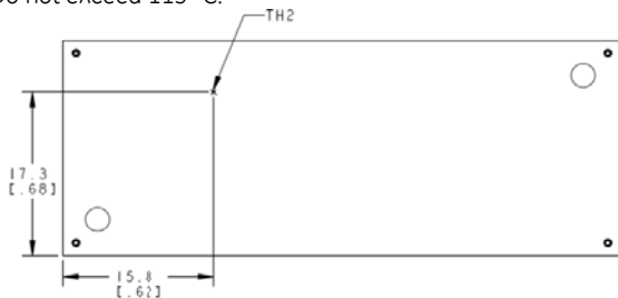
Figure 20. Location of the thermal reference temperature TH 2 for Baseplate module. Do not exceed 110 °C.
