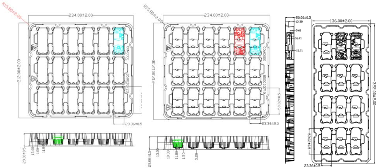
Open Frame Through Hole Pin Module Tray Figure 27. EBDW020 Packaging Tray
