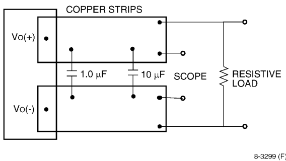
Figure 13. Input Reflected Ripple Current Test Setup.
