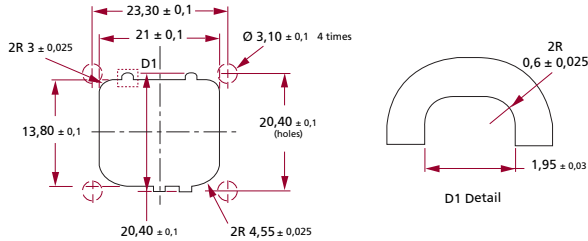
GENERIC DIMENSIONS
