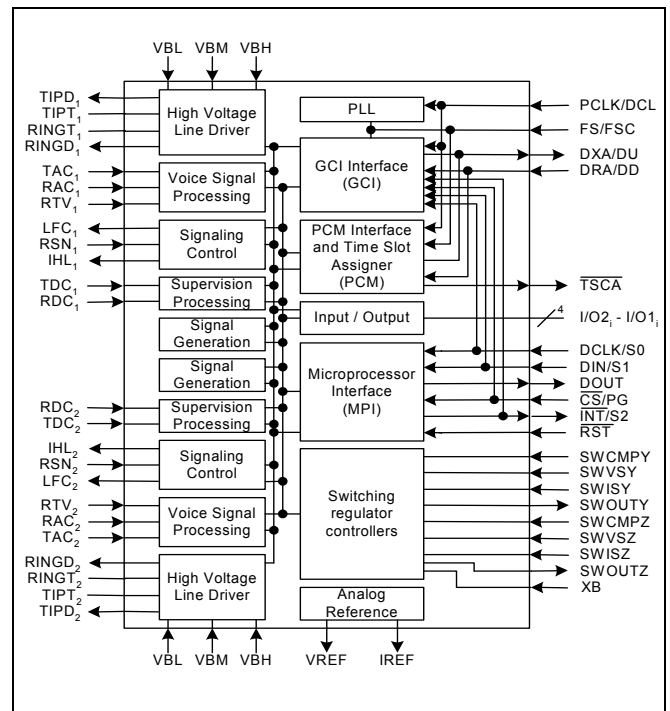
Figure 1 - VoicePort Device Block Diagram
