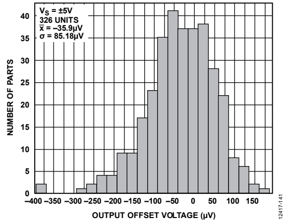
Figure 38. Differential Output Offset Voltage
