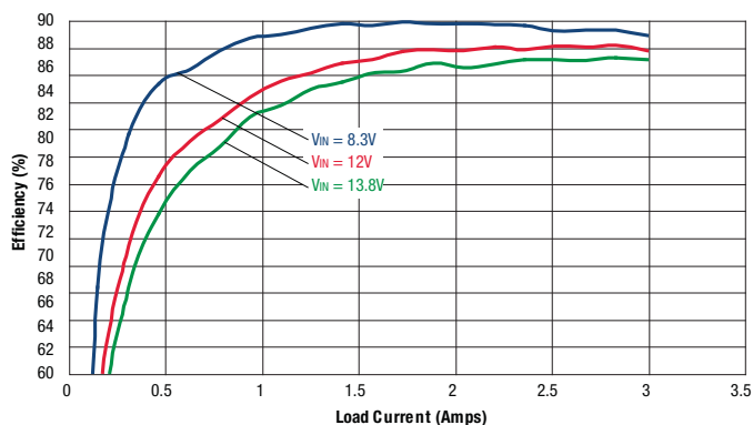
Efficiency vs. Line Voltage and Load Current @ +25°C (V OUT = 1.8V)
