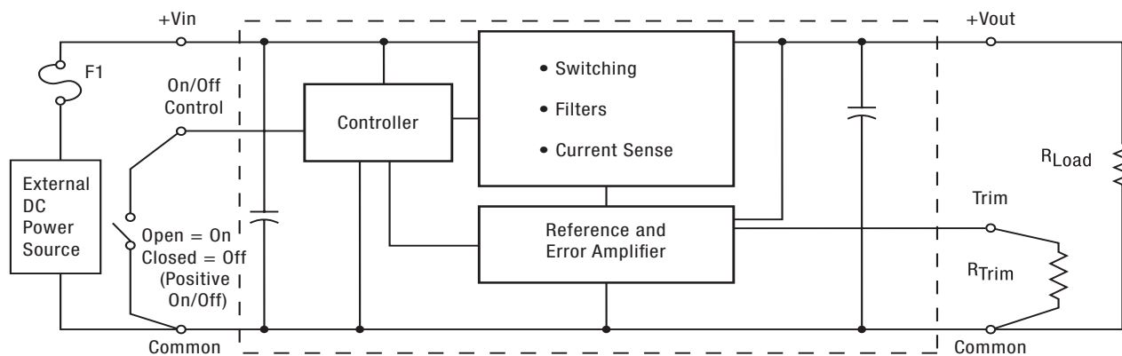
Connection Diagram
