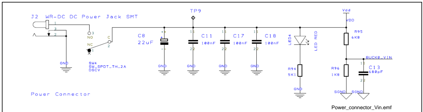
Figure 4 Synchronous buck converter power connector and Vin detail
