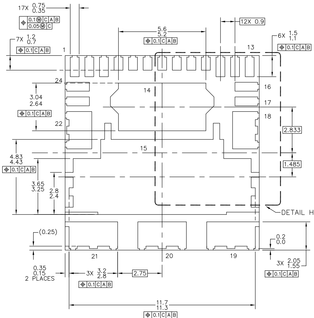
VIEW M-M
