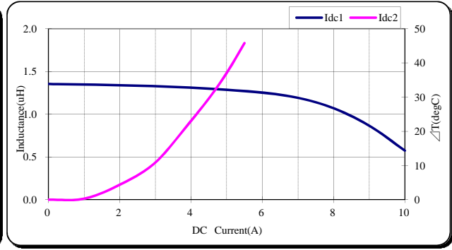
TDK' PartNo.:VLS5045EX-2R2N
