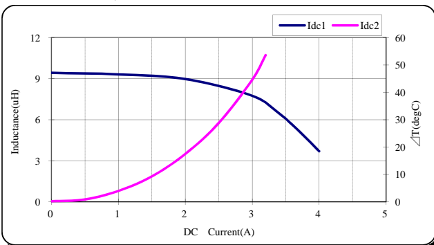
TDK' PartNo.:VLS5045EX-100M
