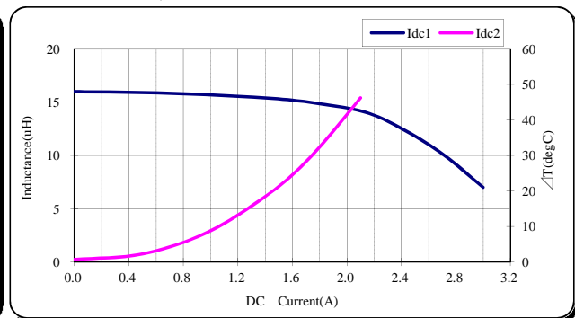
TDK' PartNo.:VLS5045EX-150M
