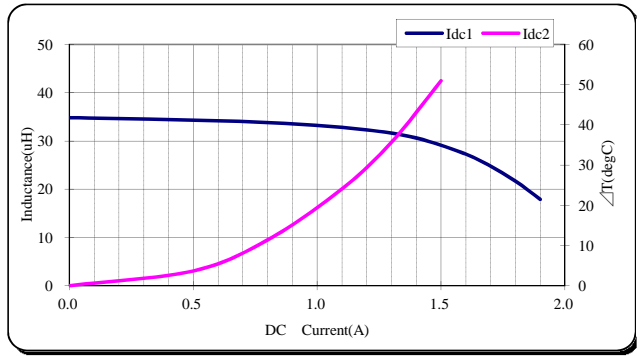
TDK' PartNo.;VLS5045EX-680M
