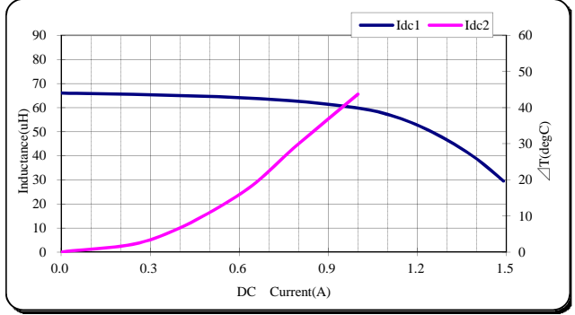
TDK' PartNo.;VLS5045EX-680M
