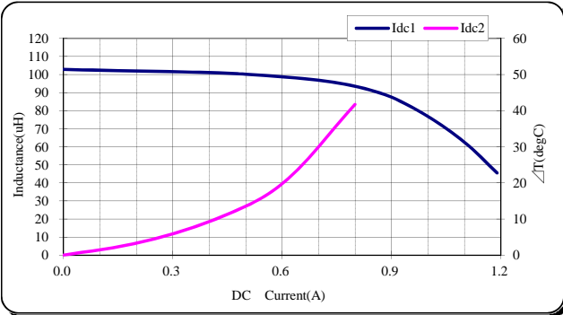
TDK' PartNo.;VLS5045EX-101M
