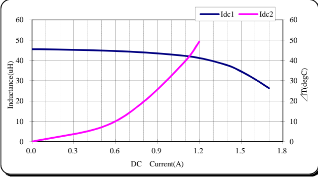
TDK' PartNo.;VLS5045EX-470M
