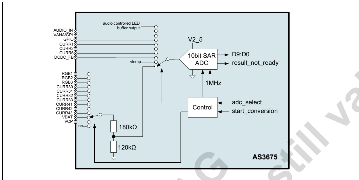
Figure 26. ADC Circuit
