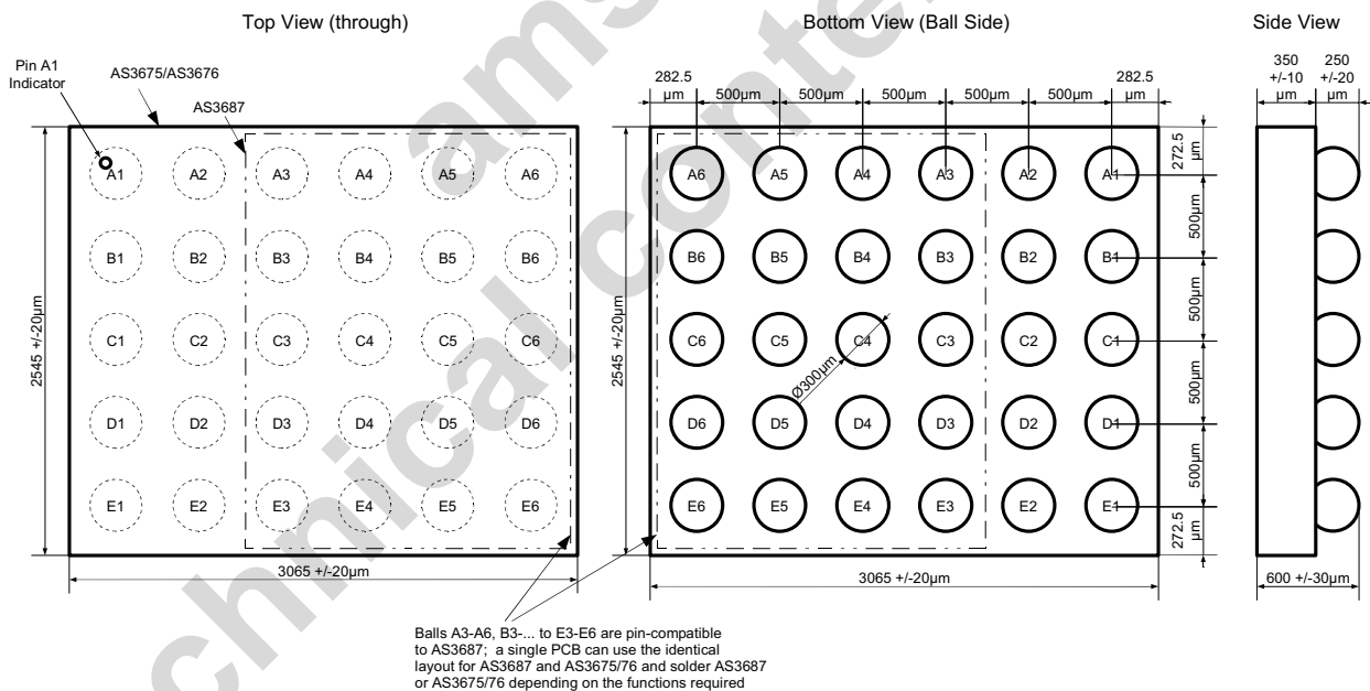
Figure 42. WL-CSP30 3x2.5mm 6x5 Balls Detail Dimensions
