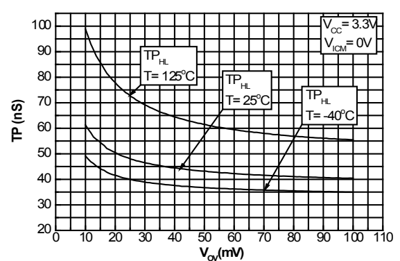
Figure 18. Propagation delay (HL) vs. overdrive at V_{cc} = 3.3V , V_{ictm} = 0V
