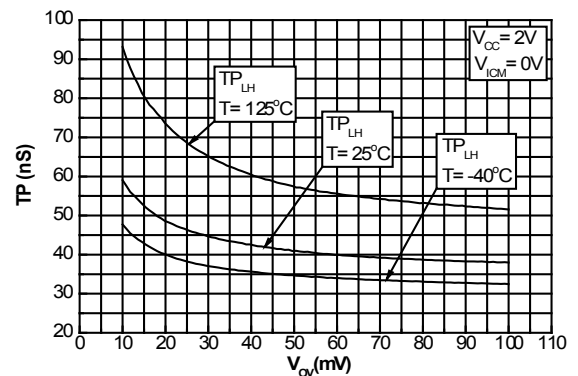
Figure 16. Propagation delay (LH) vs. overdrive at V_{cc} = 2V , V_{ictm} = 0V
