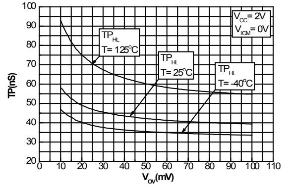
Figure 14. Propagation delay (HL) vs. overdrive at V_{cc} = 2V , V_{ictm} = 0V
