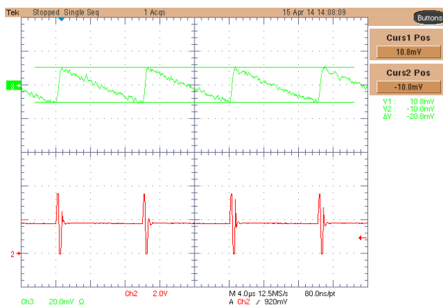
Figure 12. Output Ripple Voltage in PFM Mode ( V_{IN} = 3.6\text{ V} , V_{OUT} = 1.8\text{ V} , I_{OUT} = 10\text{ mA} , L = 1\ \mu\text{H} , C_{OUT} = 10\ \mu\text{F} )
