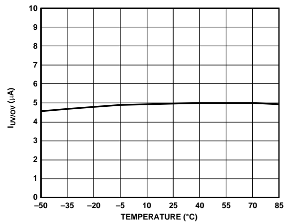
Figure 30. I UV/OV vs. Temperature
