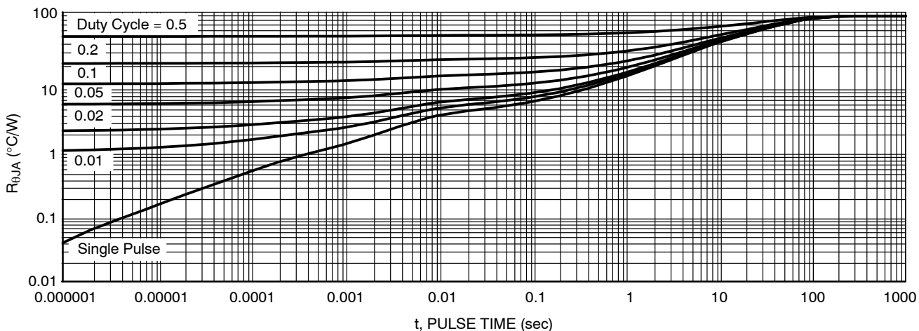
Figure 5. Thermal Response
