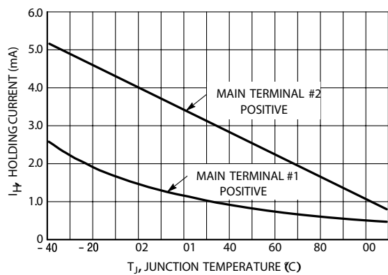
Figure 15. Typical Holding Current Variation
