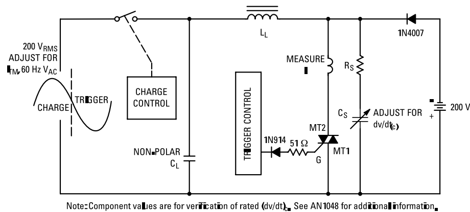
Figure 10. Simplified Test Circuit to Measure the Critical Rate of Rise of Commutating Current ( di/dt )
