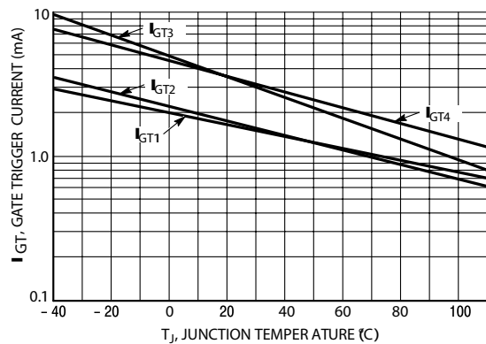
Figure 14. Typical Gate Trigger Current Variation
