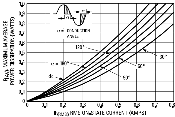
Figure 8. Power Dissipation
