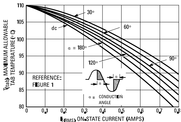
Figure 7. Current Derating Reference: MT2 Tab
