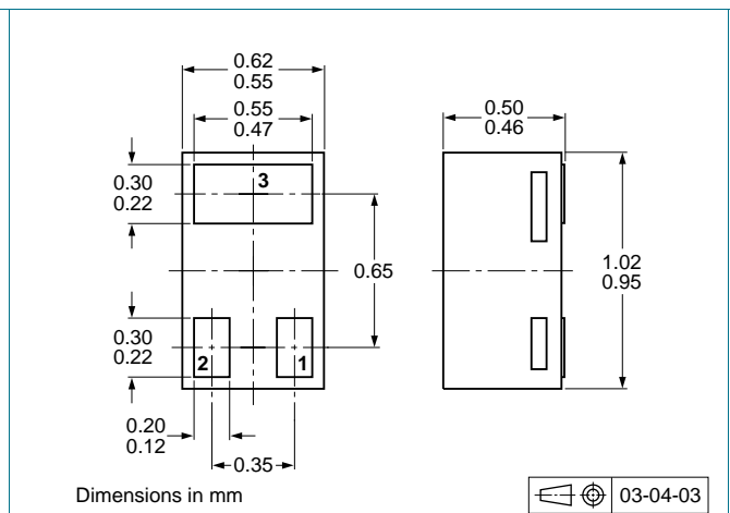
Fig 13. Package outline PDTA124EM (SOT883/SC-101)
