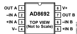
Figure 4. 8-Lead SOIC
