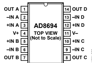
Figure 5. 14-Lead SOIC
