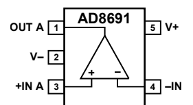
Figure 2. 5-Lead SC70
