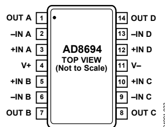
Figure 6. 14-Lead TSSOP
