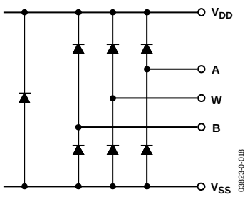
Figure 38. Maximum Terminal Voltages Set by V_{DD} and V_{SS}
