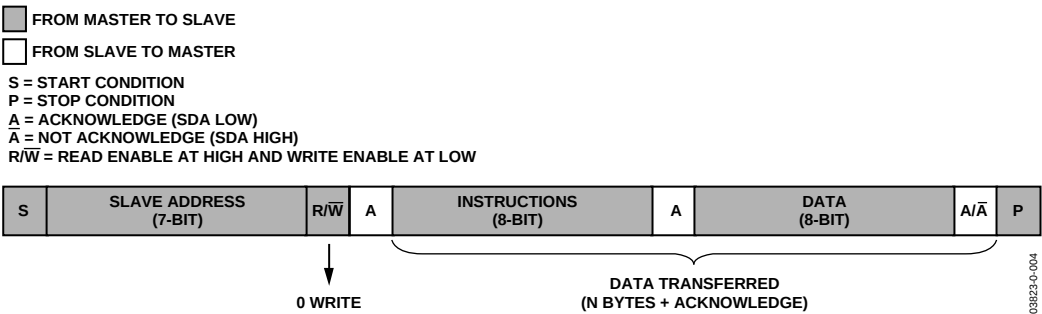
Figure 24. I 2 C—Master Writing Data to Slave
