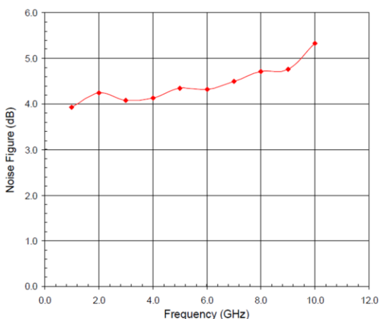
Noise Figure versus Frequency at +25°C
