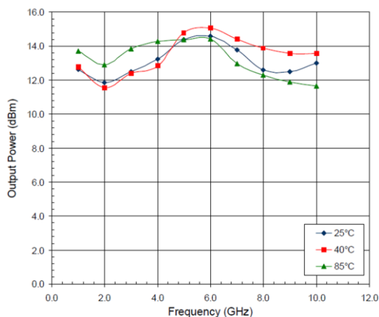
Output P1dB versus Frequency Across Temperature
