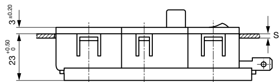
Variants 6424.0X5X.XX Mounting hole: 57 \pm 0.2 \times 27.6 \pm 0.2 A: Quick-connect terminal 6.3 \times 0.8 mm: 18.1 mm A: Solder terminal 3.5 \times 0.8 mm: 13.3 mm S: Panel thickness
