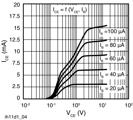
Fig. 3 - Output Characteristics
