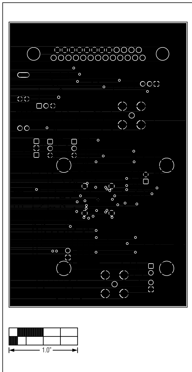
Figure 4. MAX2140 EV Kit PCB Layout—Layer 2
