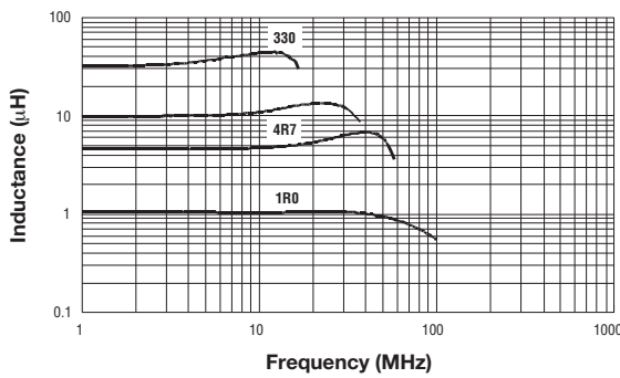
Inductance Characteristics
