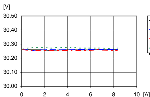
Output voltage vs. load current at T_{ref} = +25^{\circ}\text{C}
