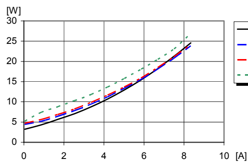
Dissipated power vs. load current and input voltage at T_{ref} = +25^{\circ}\text{C}
