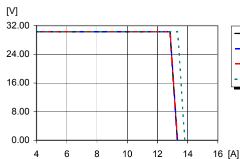
Output voltage vs. load current at I_O > \max I_O , T_{ref} = +25^{\circ}\text{C}
