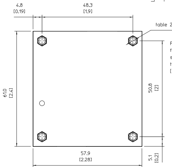
Recommended Footprint - TOP VIEW
