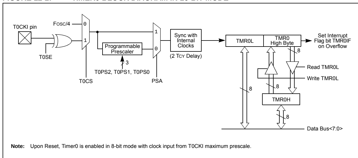
FIGURE 12-2: TIMER0 BLOCK DIAGRAM IN 16-BIT MODE
