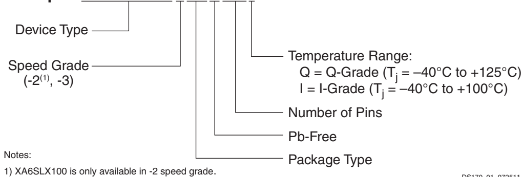
Figure 1: XA Spartan-6 FPGA Ordering Information
