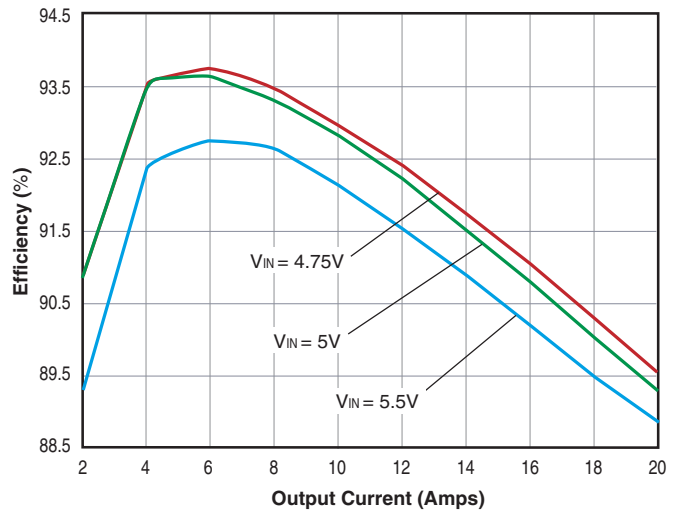
UNR-3.3/20-D5 Efficiency vs. Load @ 25°C Ambient
