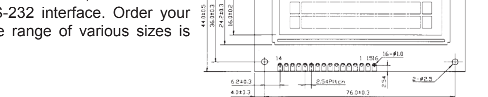
all dimensions in mm
