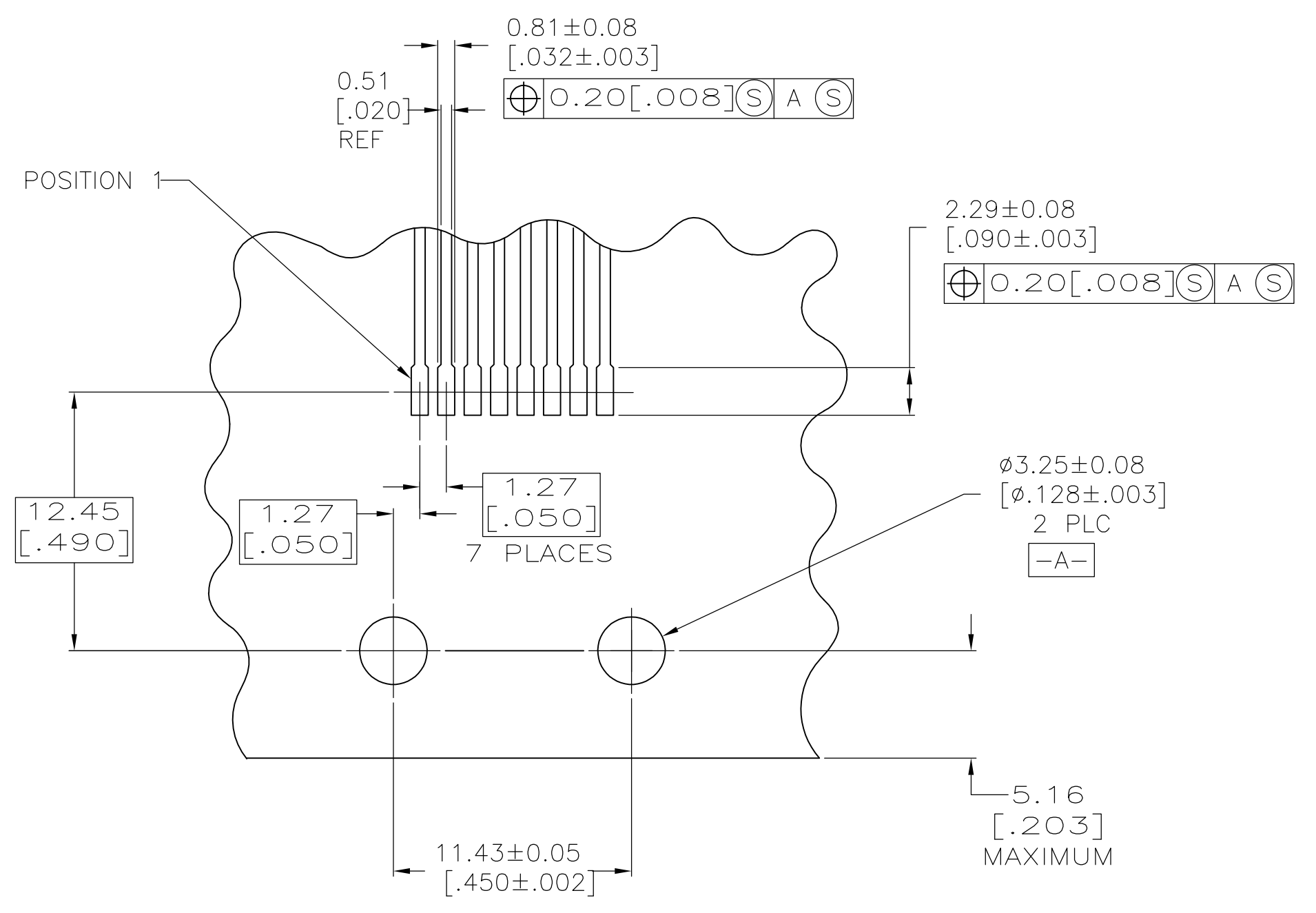
RECOMMENDED PRINTED CIRCUIT BOARD COMPONENT SIDE
