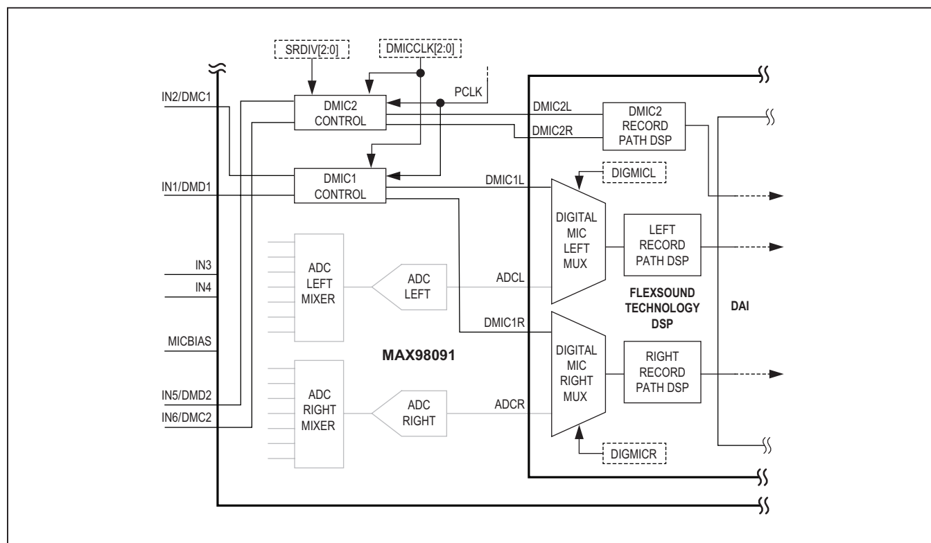
Figure 7. Digital Microphone Input Functional Diagram
