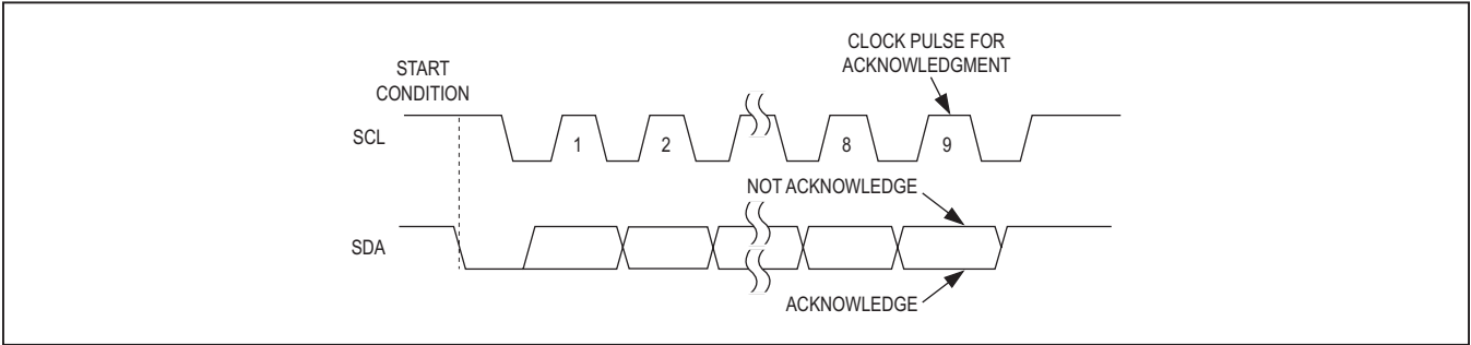
Figure 49. Acknowledge Timing
