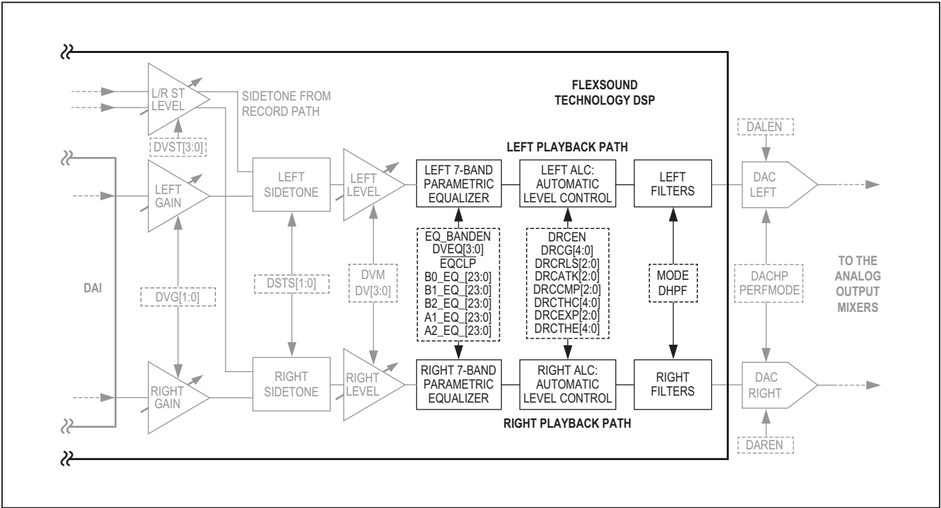
Figure 26. Playback Path DSP
