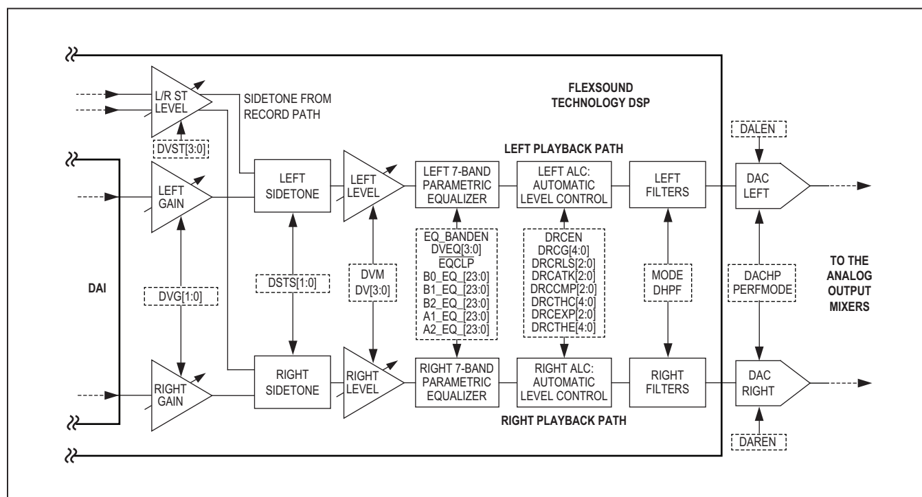
Figure 24. Playback Path Block Diagram
