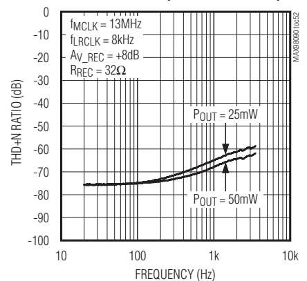
TOTAL HARMONIC DISTORTION vs. FREQUENCY (DAC TO RECEIVER)
