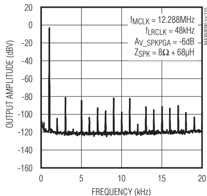
INBAND OUTPUT SPECTRUM, -3dBFS INPUT (DAC TO SPEAKER)
