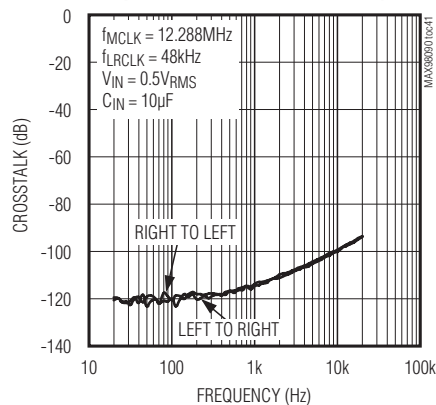
CROSSTALK vs. FREQUENCY (INPUT DIRECT TO ADC MIXER)
