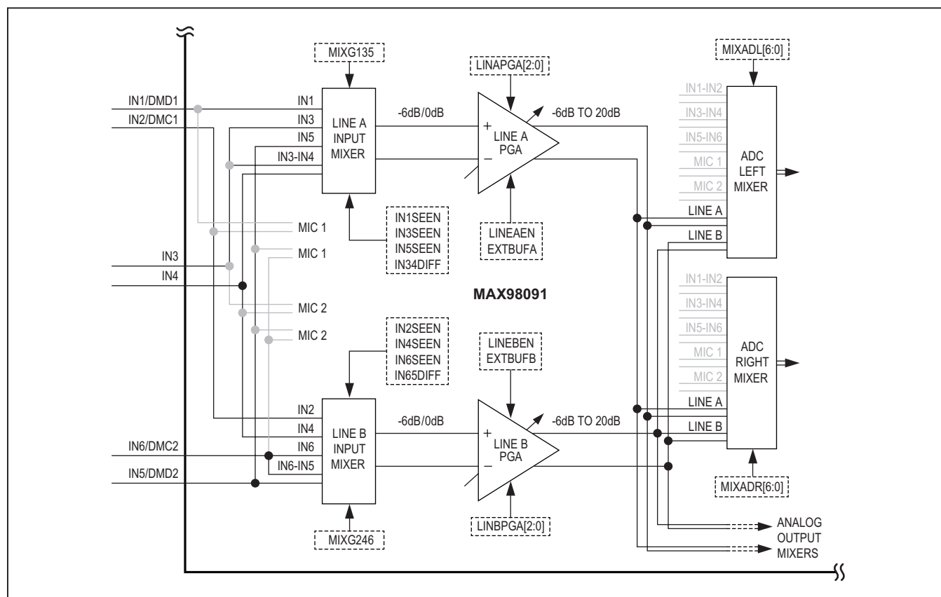
Figure 10. Analog Line Input Functional Diagram
