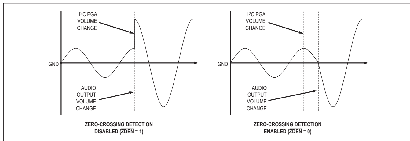
Figure 43. Zero-Crossing Detection
