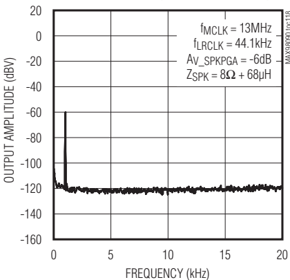
INBAND OUTPUT SPECTRUM, -60dBFS INPUT (DAC TO SPEAKER)
