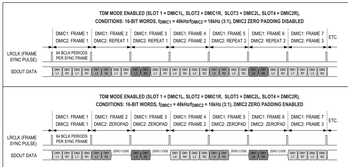
Figure 8. Secondary Record Path Sample Rate Division
