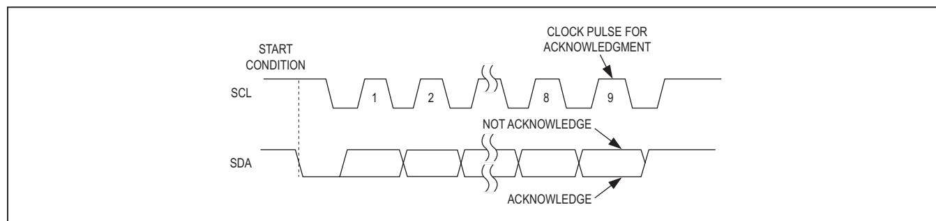
Figure 49. Acknowledge Timing
