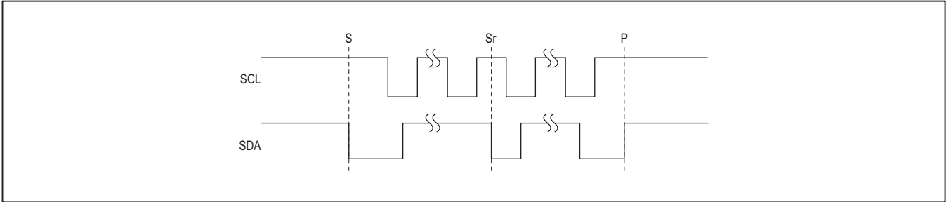
Figure 48. START, STOP, and REPEATED START Conditions
