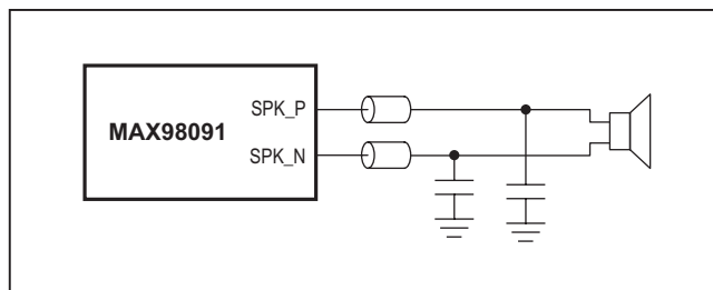
Figure 56. Optional Class D Ferrite Bead EMI Filter
