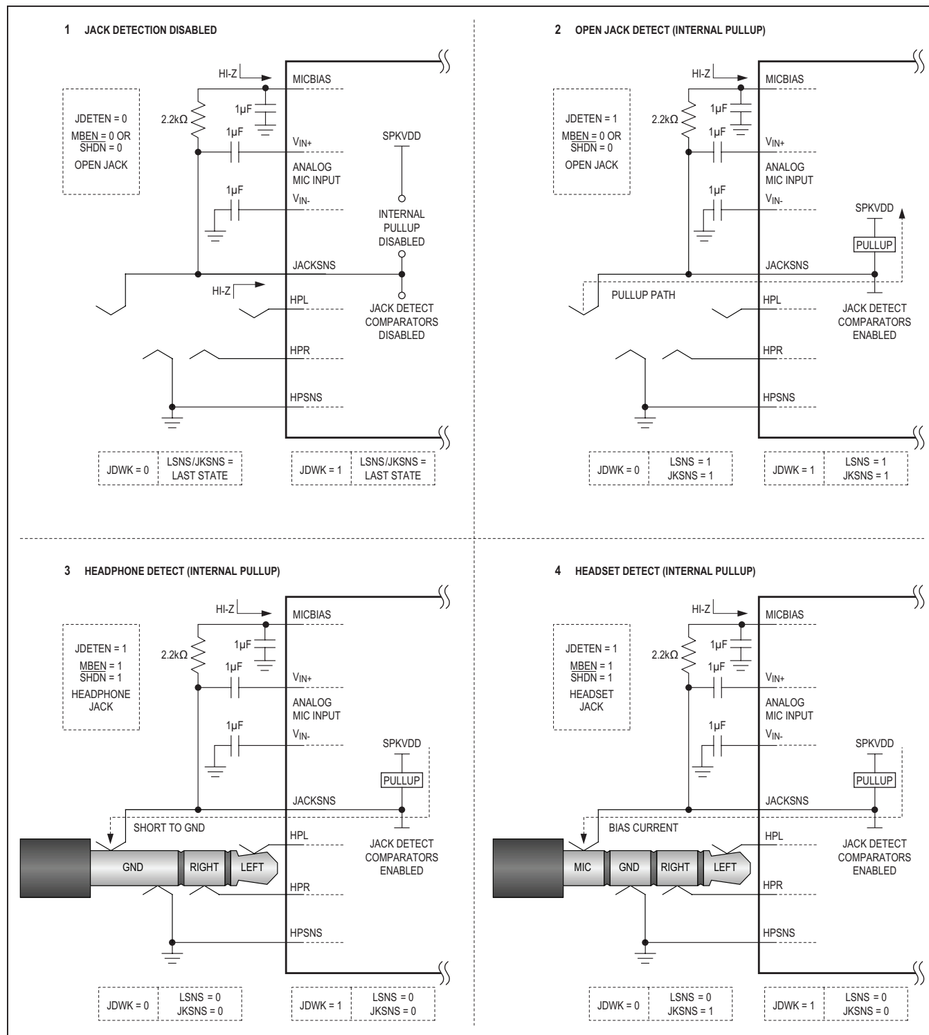
Figure 45. Jack Detection Cases with Internal Pullup Resistance
