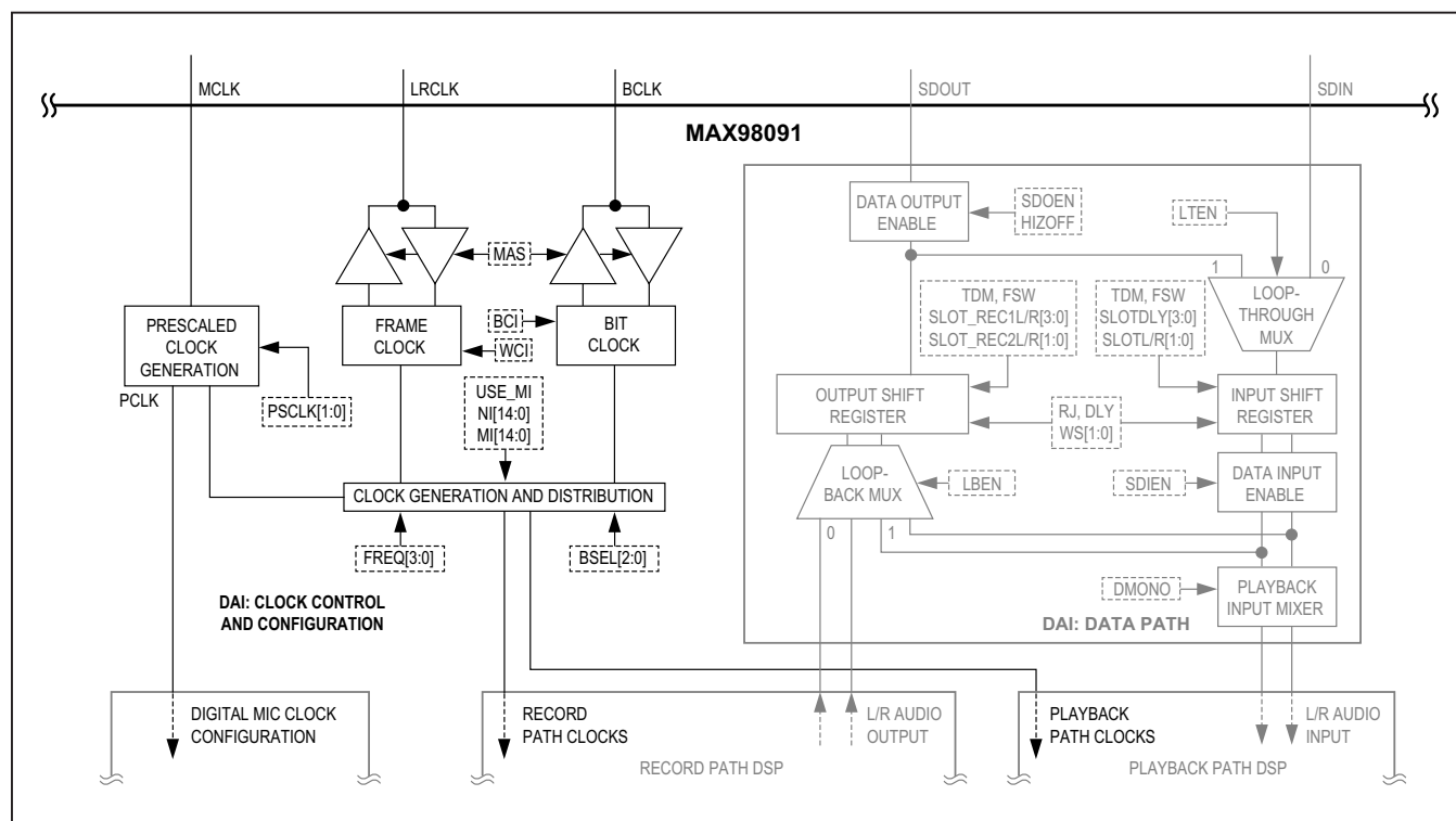
Figure 17. DAI Clock Control and Configuration Section
