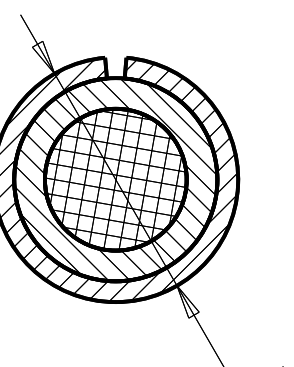
INSULATION CRIMP DIMENSIONS
