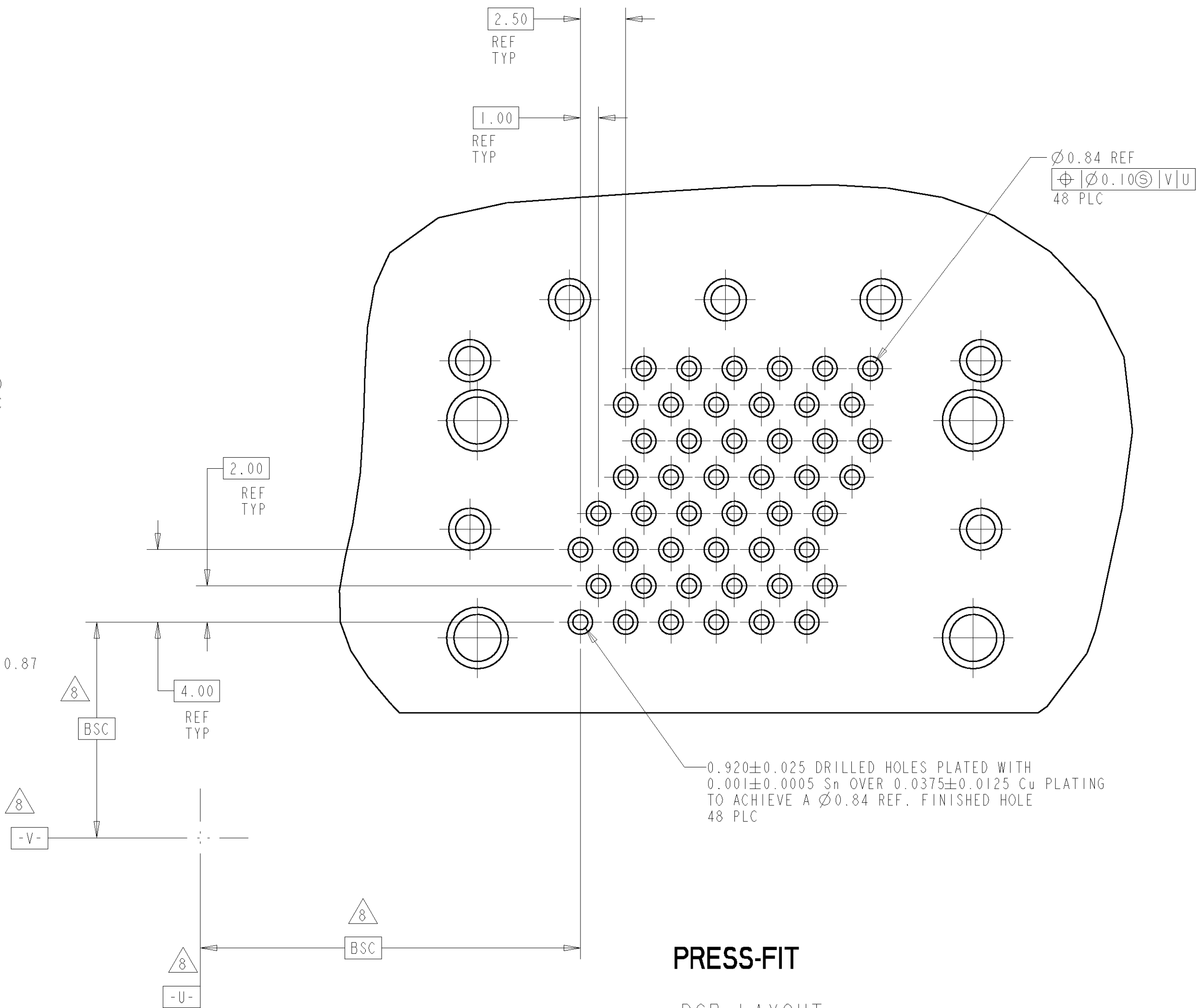
PCB LAYOUT SAME AS -1 EXCEPT AS NOTED SCALE 5:1
