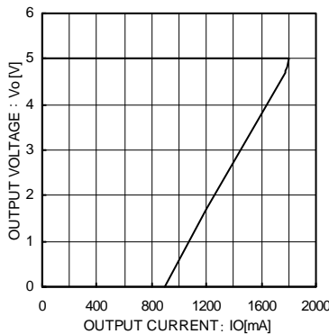
Fig.17 Load Regulation
