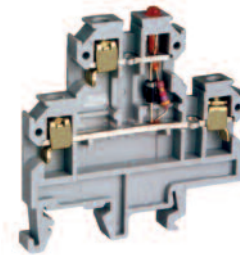
AC/ DC voltage indicator with LED
