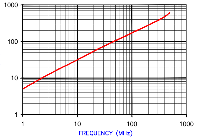
AGILENT E4991A Impedance/Material Analyzer HP 16092A-Test Fixture TEST REF. 3097
