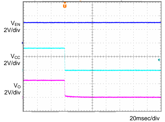
Fig.14 OFF sequence 1 Co=1μF, Ta=105°C
