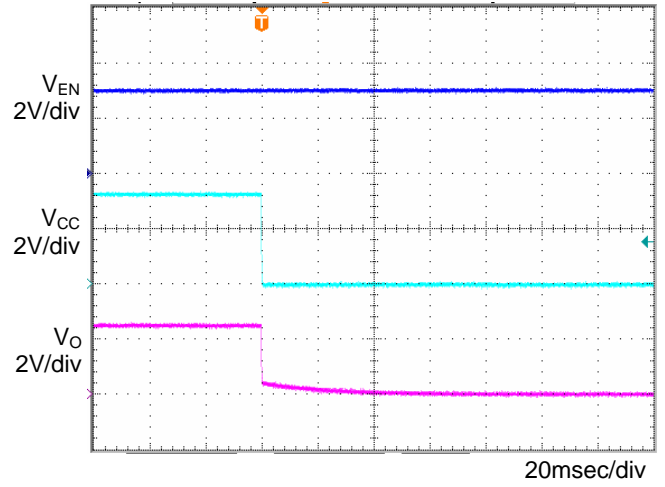
Fig.12 OFF sequence 1 C_o = 1\mu\text{F} , T_a = -40^\circ\text{C}
