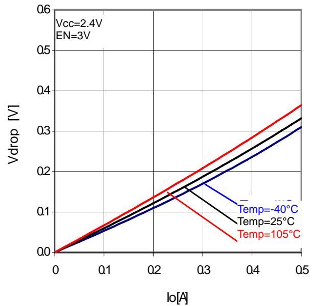
Fig.34 Minimum dropout Voltage 1 ( V_{CC}=2.4V )
