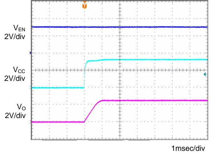
Fig.10 Input sequence 1 Co=1μF,Ta=25°C
