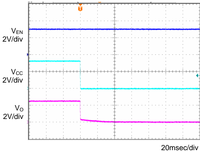
Fig.13 OFF sequence 1 C_o = 1\mu\text{F} , T_a = 25^\circ\text{C}
