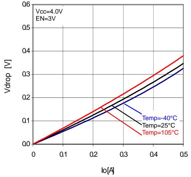
Fig.36 Minimum dropout Voltage 3 (V CC =4.0V)
