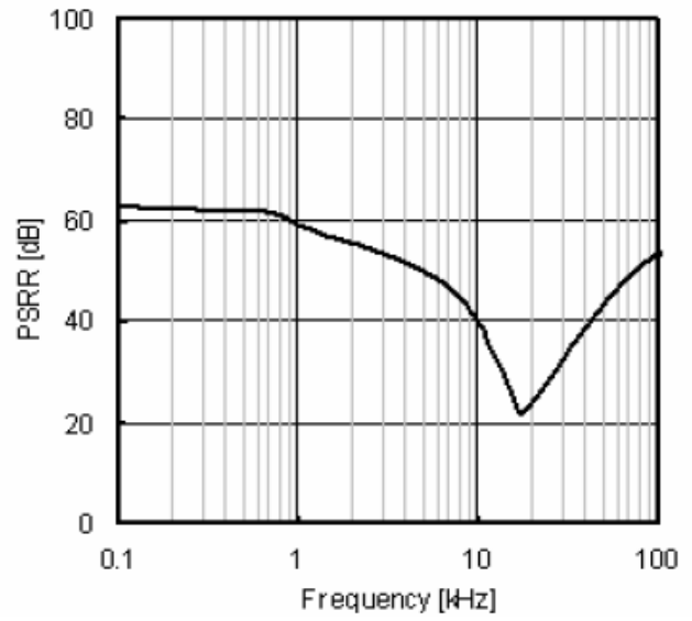
Fig.32 PSRR ( I_o=0mA )
