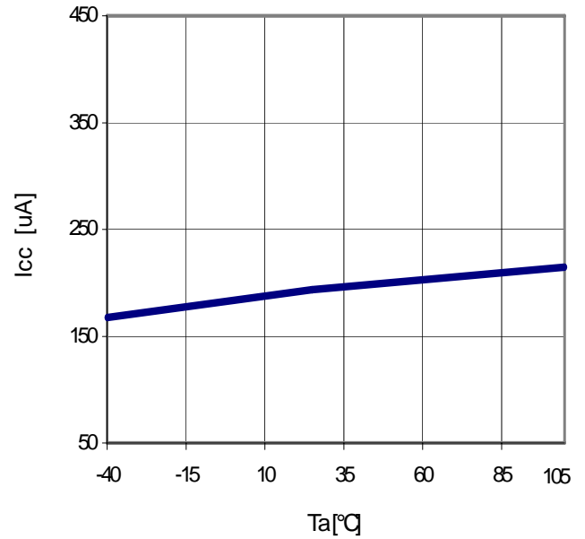
Fig.22 T_a - I_{CC}
