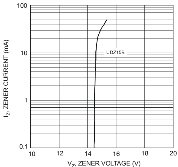
Fig. 5 Typical Zener Breakdown Characteristics, UDZ15B
