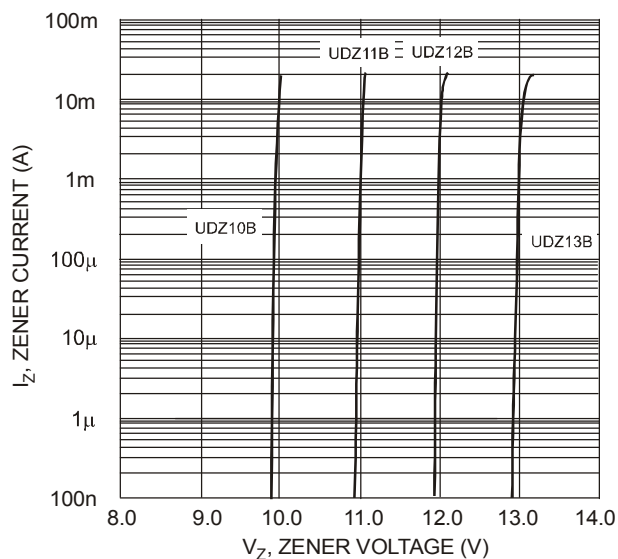
Fig. 4 Typical Zener Breakdown Characteristics, UDZ10B - UDZ13B
