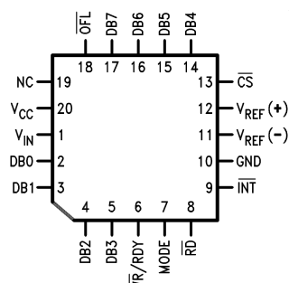
Molded Chip Carrier Package
