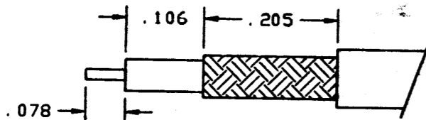
CABLE STRIPPING DIMENSIONS
