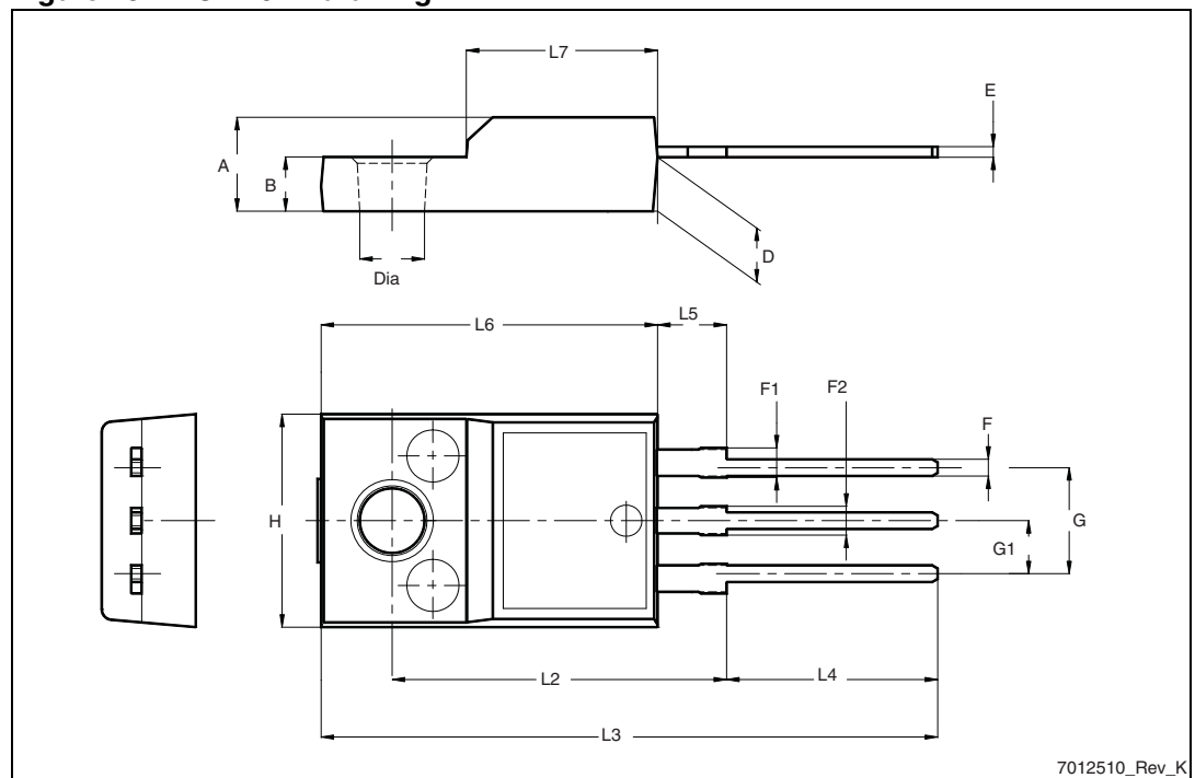
Figure 25. TO-220FP drawing
