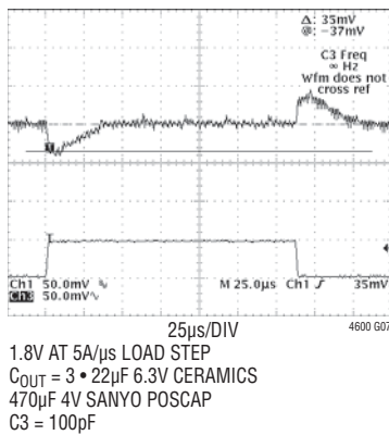
1.8V Transient Response
