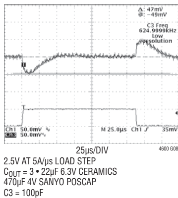
2.5V Transient Response
