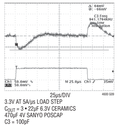
3.3V Transient Response
