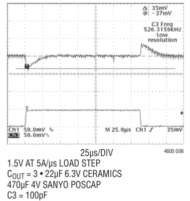
1.5V Transient Response
