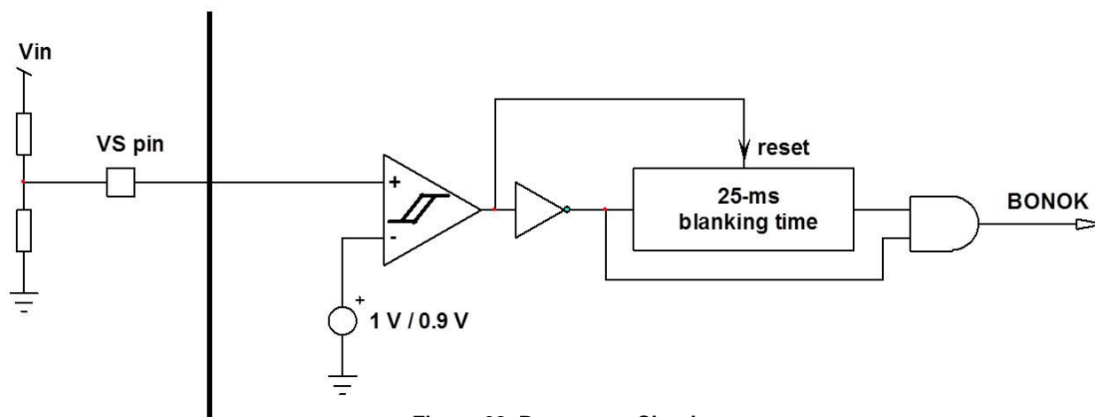
Figure 68. Brown-out Circuit
